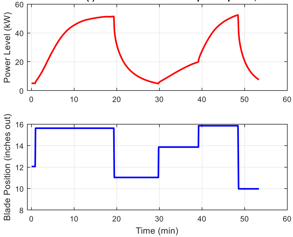
Simulated P(t) & Blade Position for Expt on April 17, 2018
