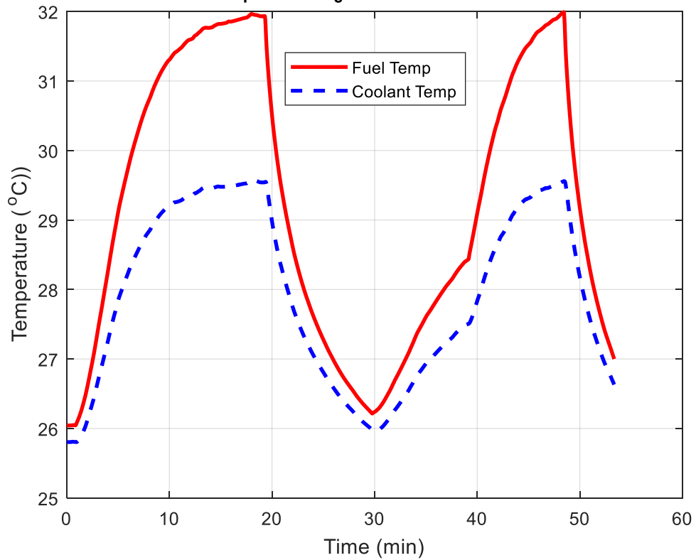
Simulated T_f(t) and T_c(t) for Expt on April 17, 2018
