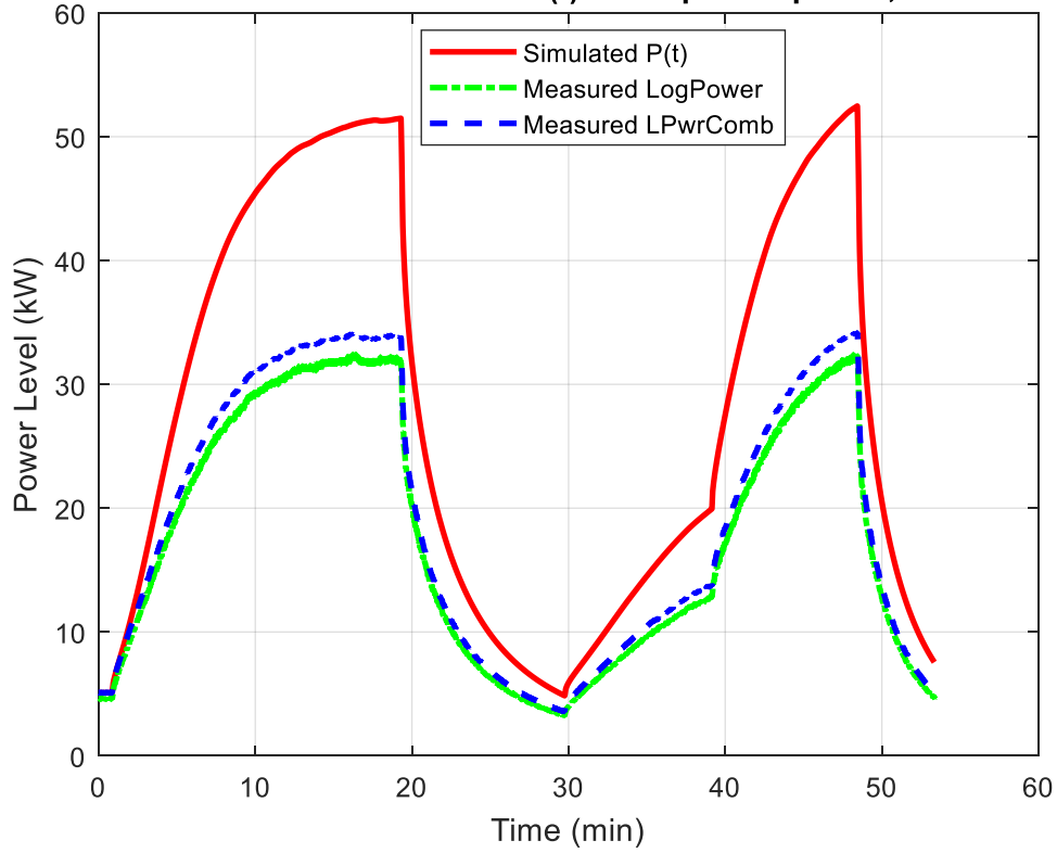
Simulated vs Measured P(t) for Expt on April 17, 2018
