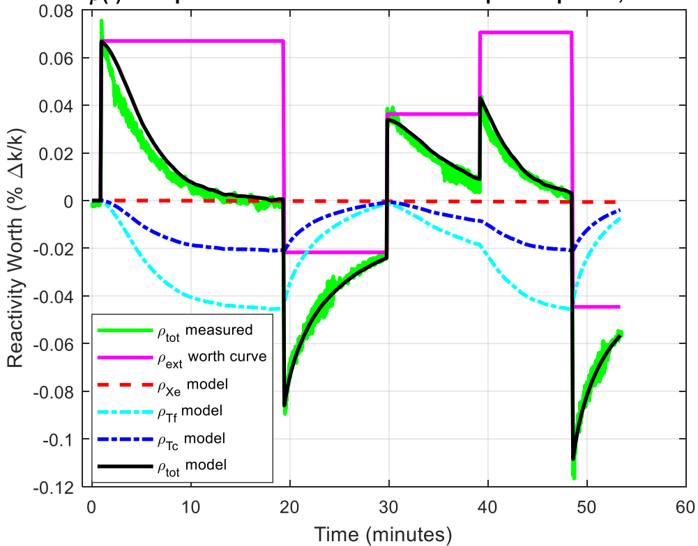
\rho(t) Components from Simulation for Expt on April 17, 2018
