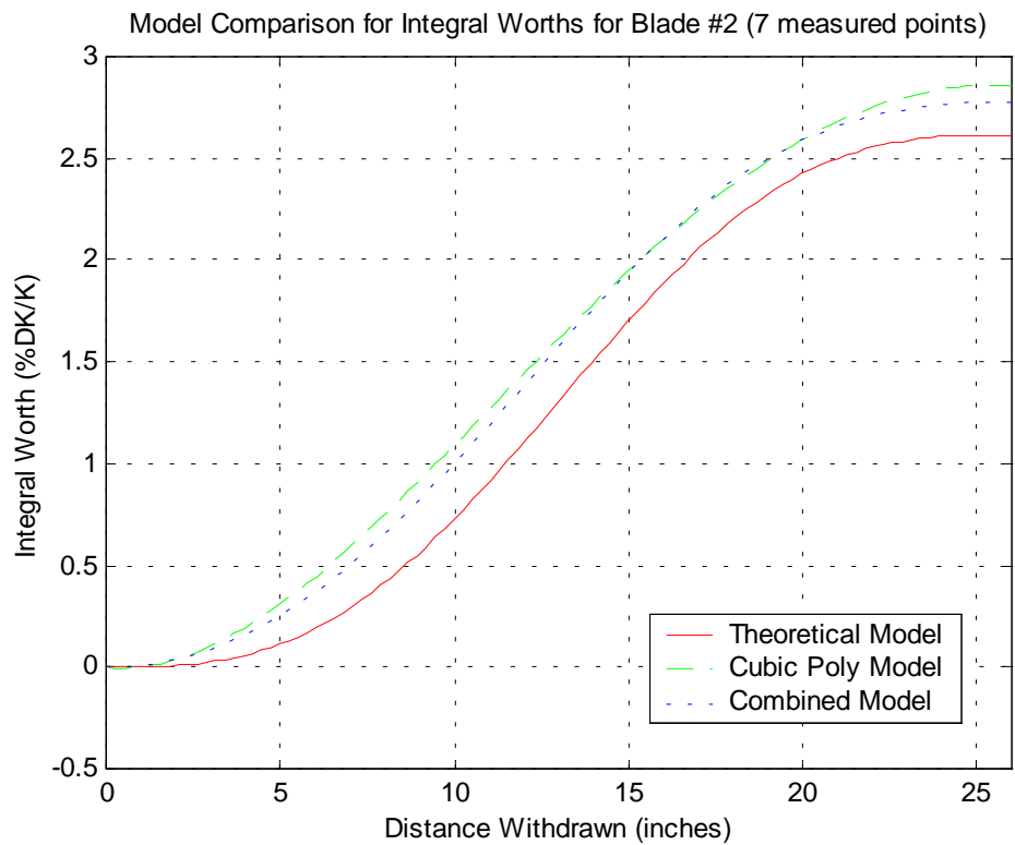
Fig. 8 Differential and integral worth curves for Blade #2.
