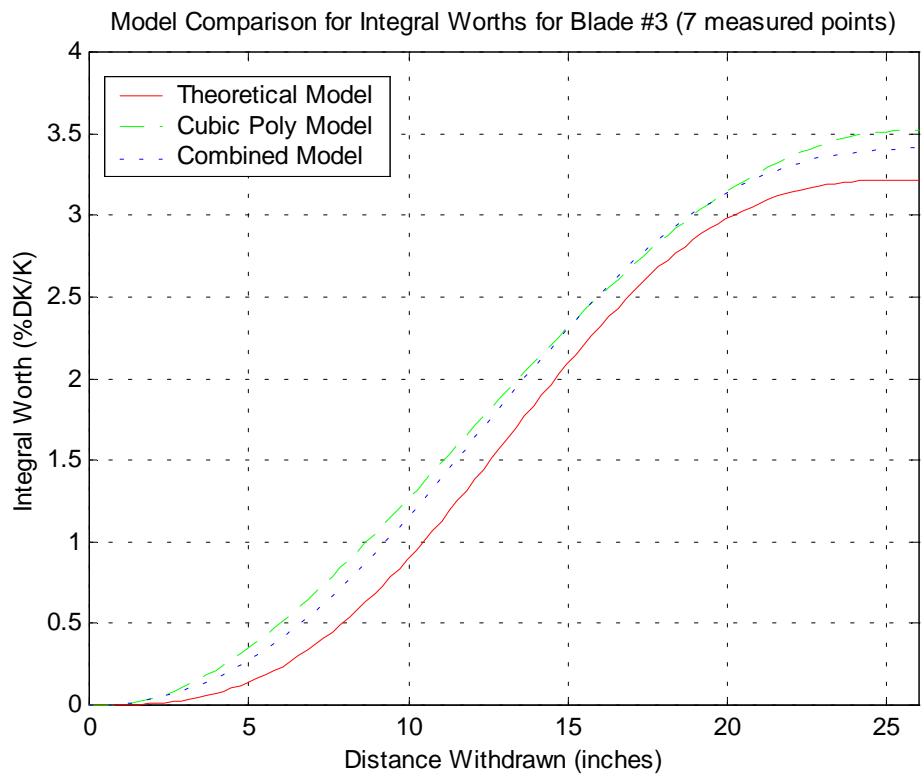
Fig. 9 Differential and integral worth curves for Blade #3.
