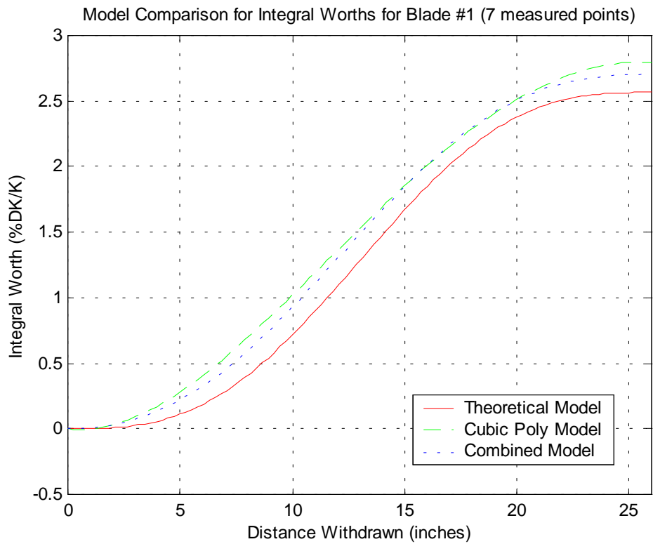
Fig. 7 Differential and integral worth curves for Blade #1.
